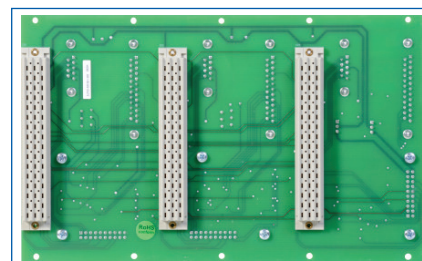
Front View Backplane A6371/xx
