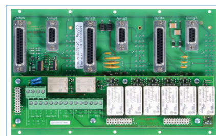
Rear View Backplane A6371/10
