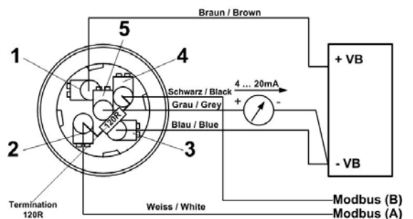
Wiring diagram
