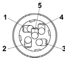
Connector plug
